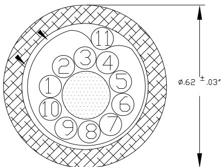
CROSS SECTIONAL VIEW
