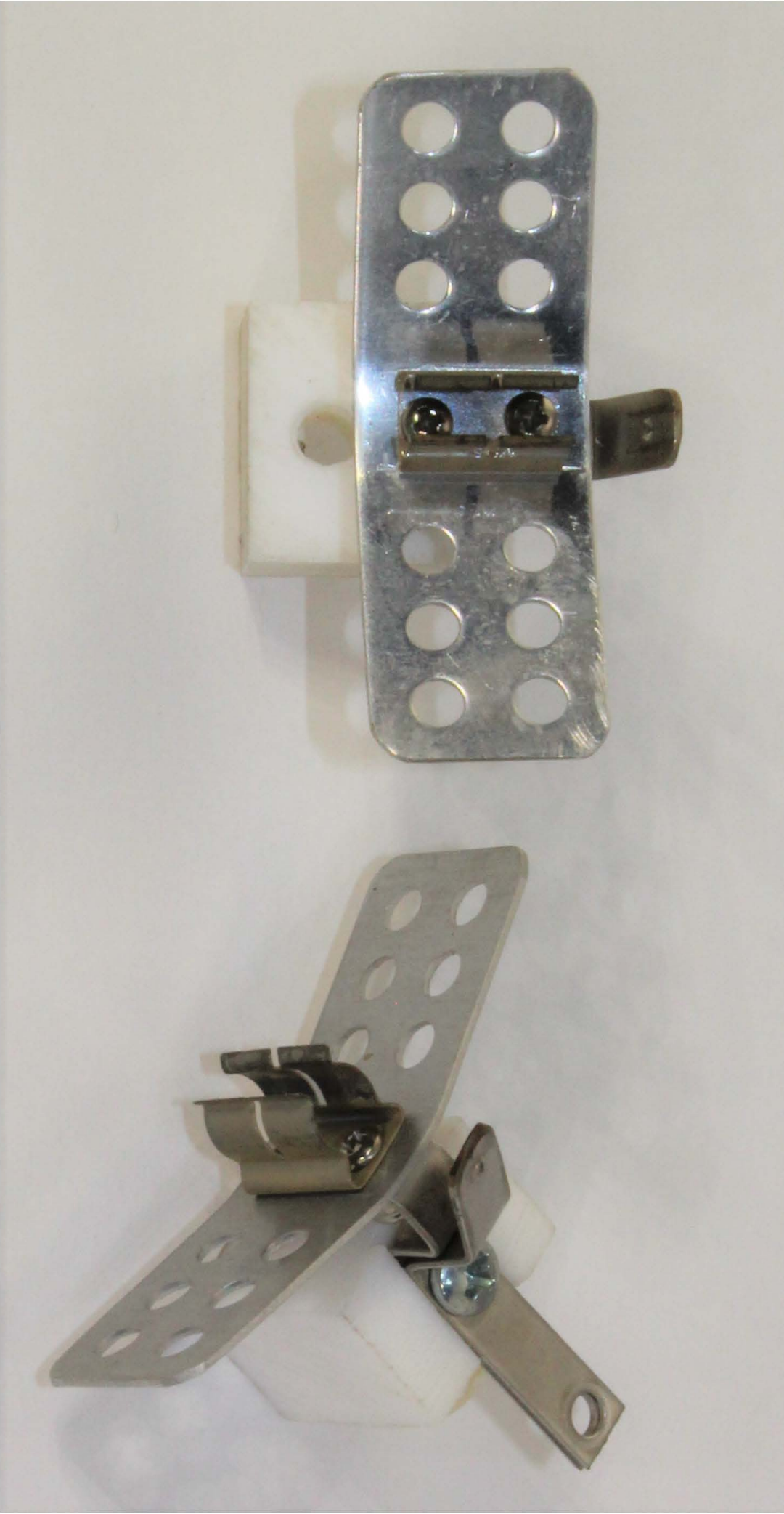
Flashtube Socket (Pair) Assembly, 277-3909
